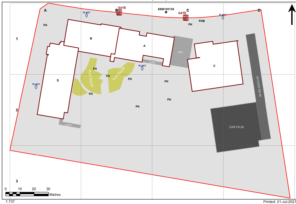
4670 - Galungara Public School Site Plan (14747)
