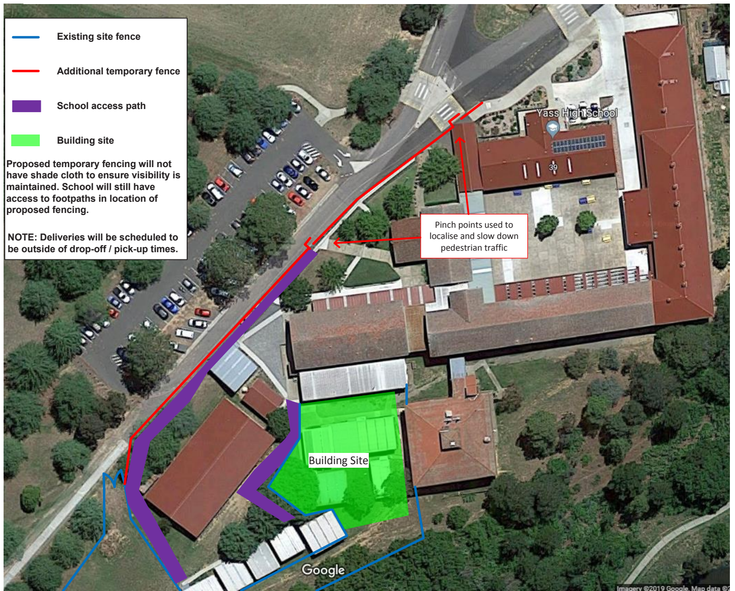
Site plan for traffic management
