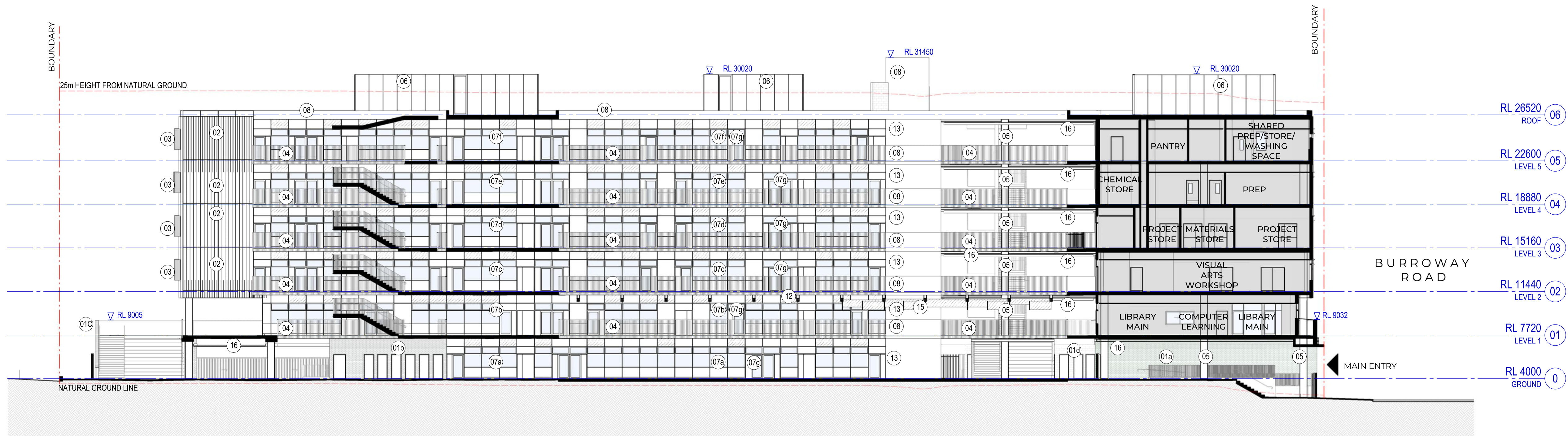
2 OVERALL SECTION 2 SCALE 1 : 200
