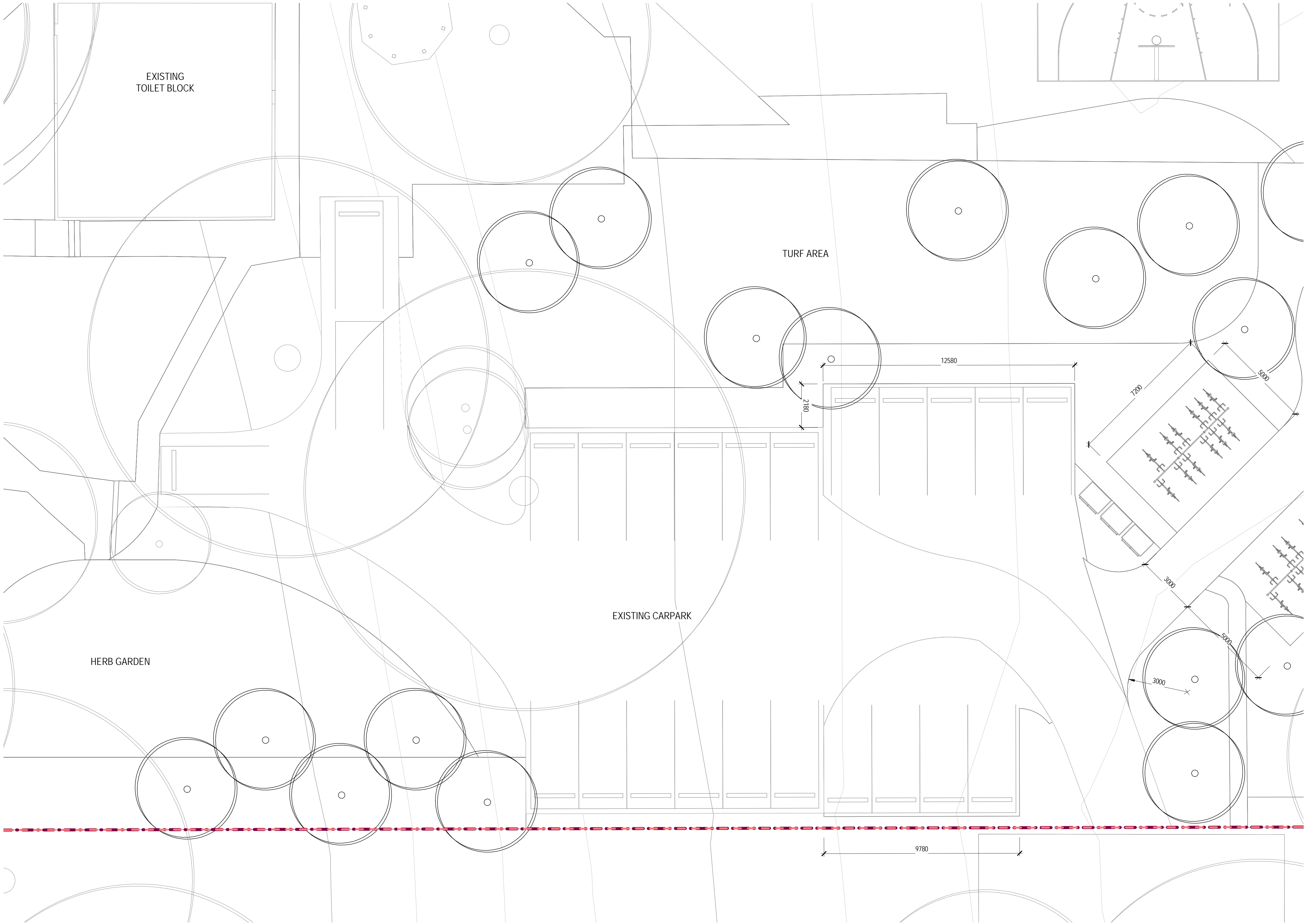
LEVELS AND SETOUT PLAN (SHEET 7 OF 8) SCALE 1 : 100
