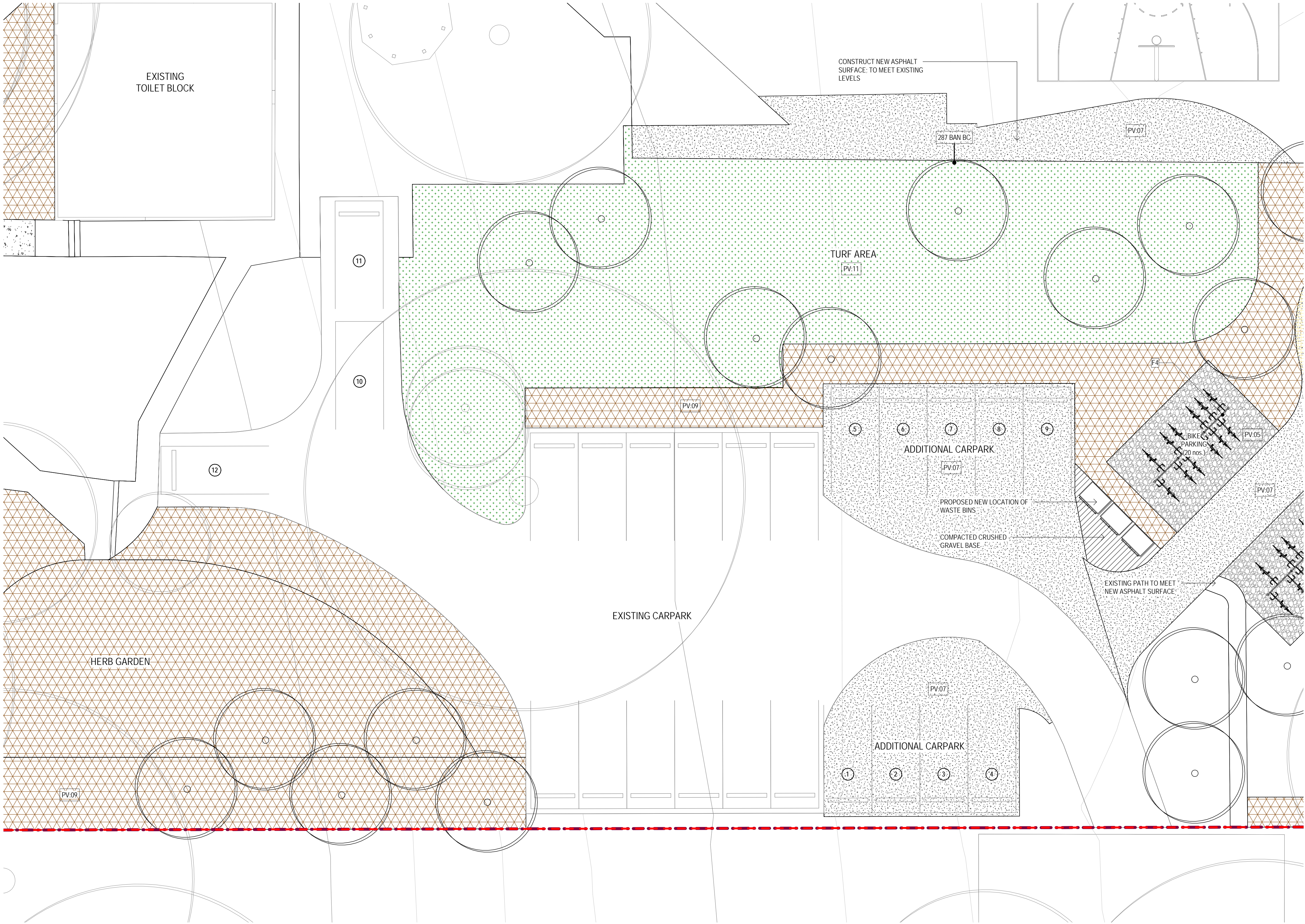
GENERAL ARRANGEMENT PLAN (SHEET 7 OF 8) SCALE 1 : 100
