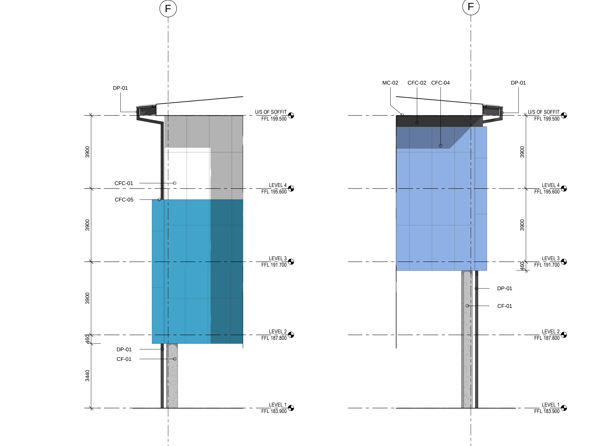
5 East Elevation - Grid 4 1 : 100
