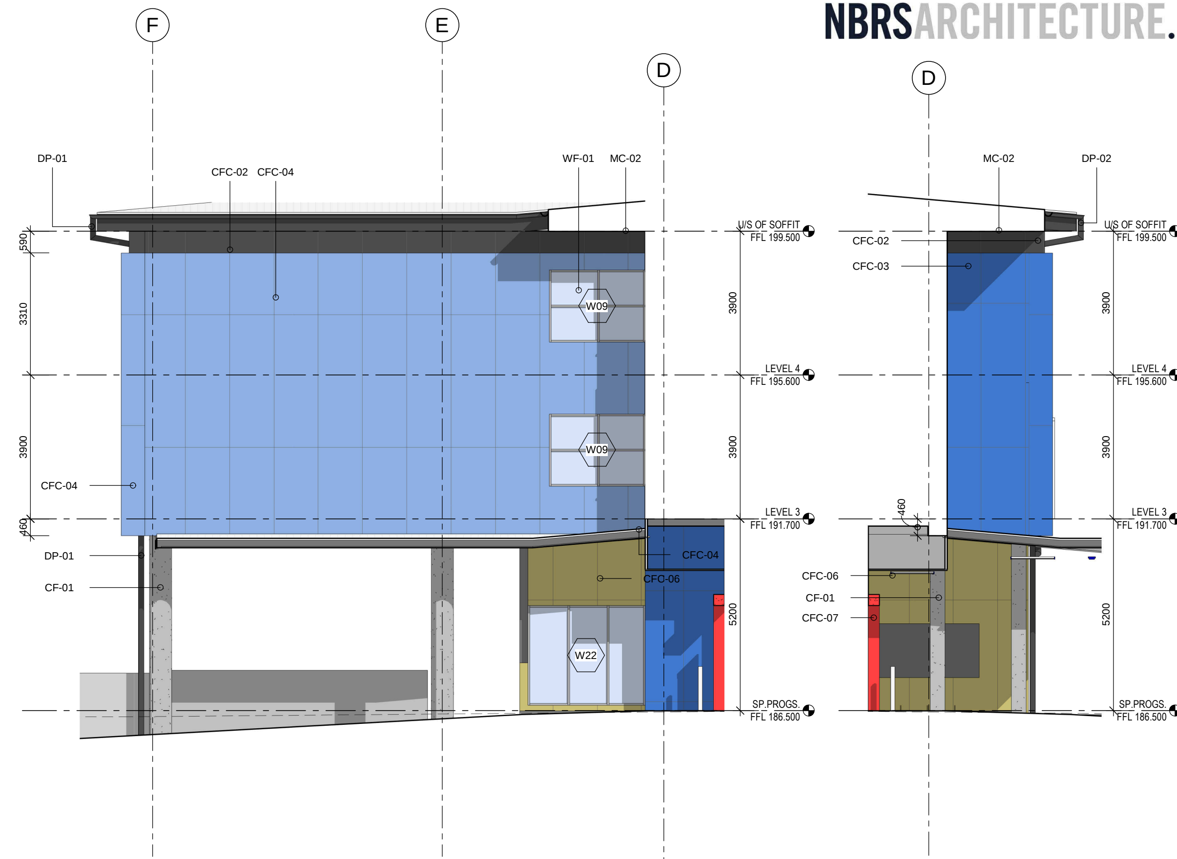
3 East Elevation - Grid 8 1 : 100
