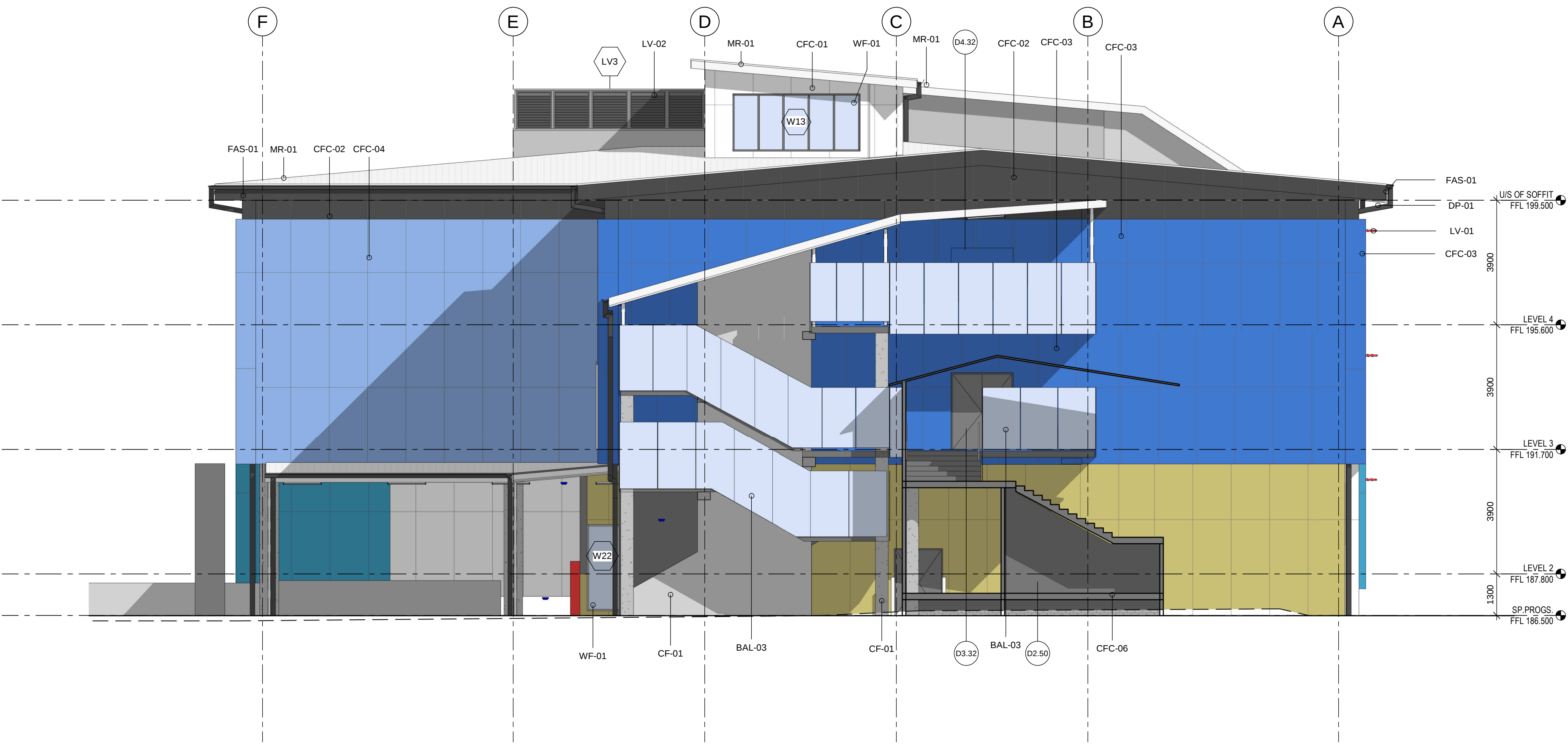
1 East Elevation 1 : 100
