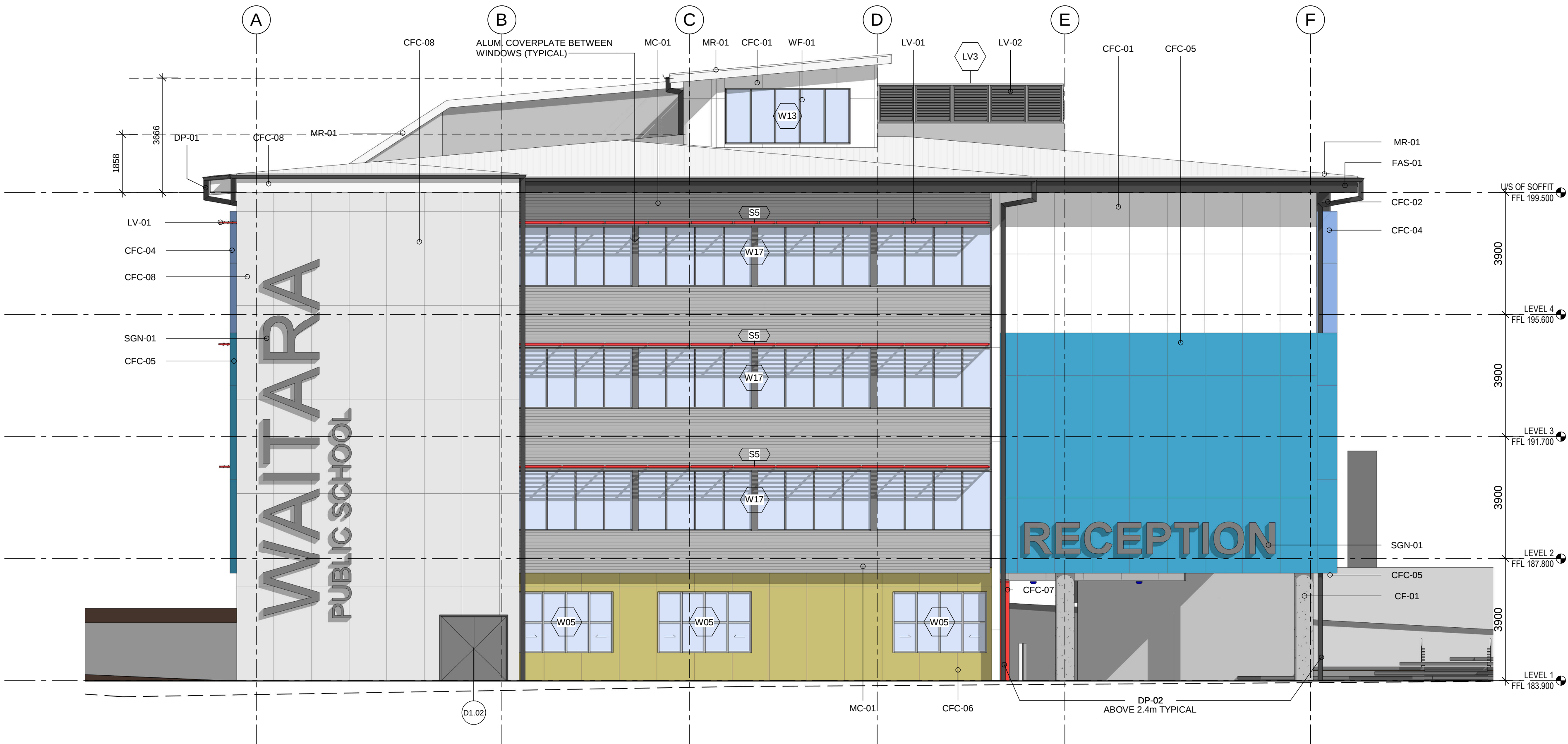
2 West Elevation 1 : 100
