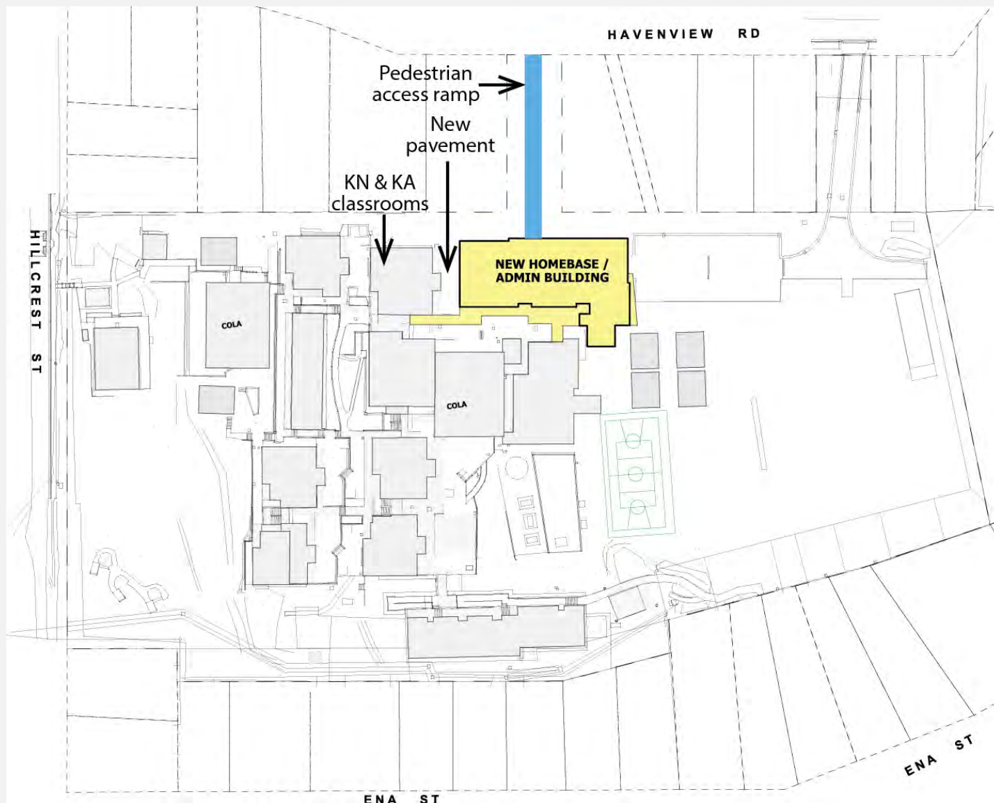
Locations of pedestrian access ramp and new pavement at Terrigal Public School
