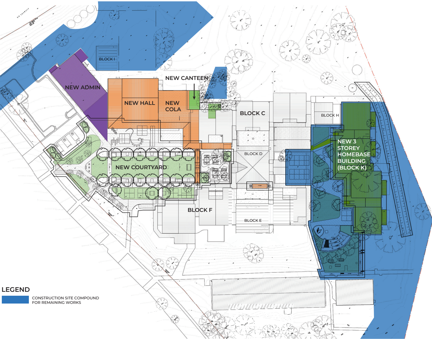
Indicative site layout map of Rutherford Public School upgrade
