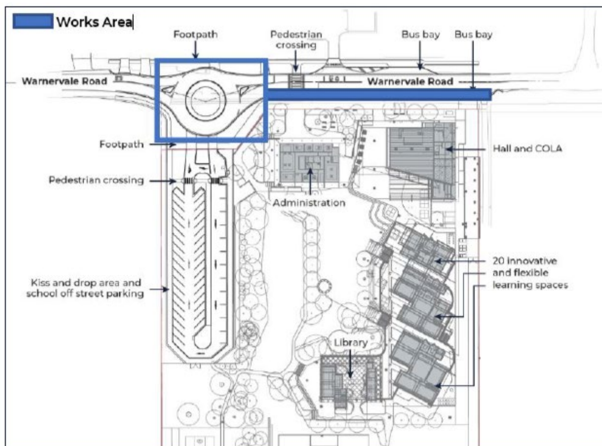
Indicative map of Warnervale Road work zone
