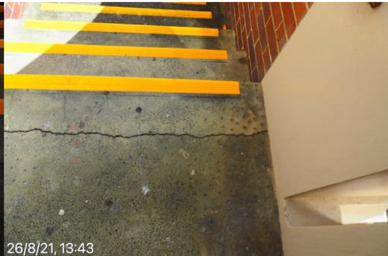
MOSMAN HIGH SCHOOL Building D North facade centre stairs to east stairs. 26 August 2021 at 13:43:47
