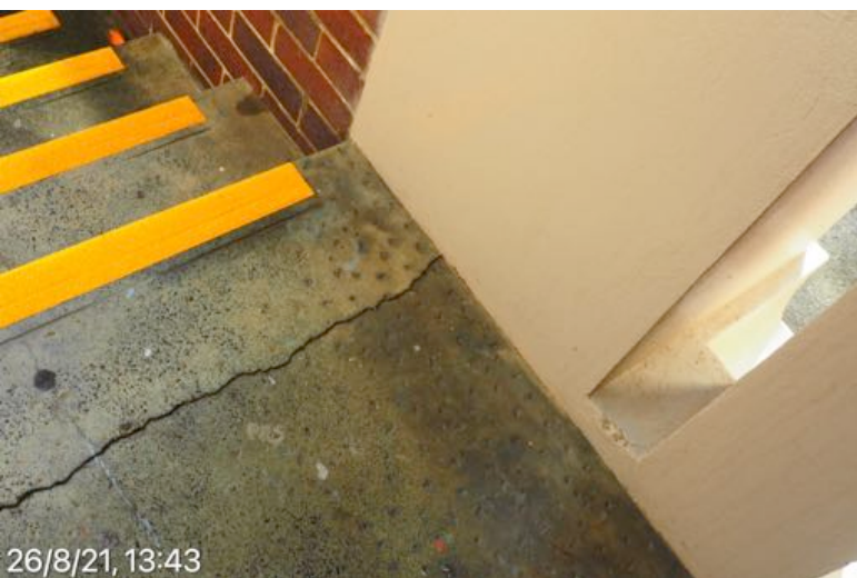
MOSMAN HIGH SCHOOL Building D North facade centre stairs to east stairs. 26 August 2021 at 13:43:26
