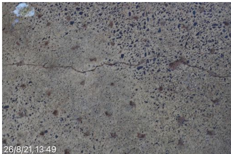
MOSMAN HIGH SCHOOL Building D North facade centre stairs to east stairs. 26 August 2021 at 13:49:42
