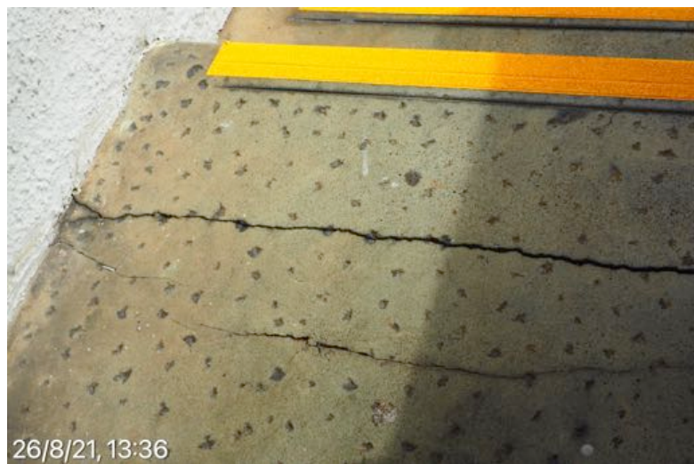
MOSMAN HIGH SCHOOL Building D North facade from west to centre stairs 26 August 2021 at 13:36:37
