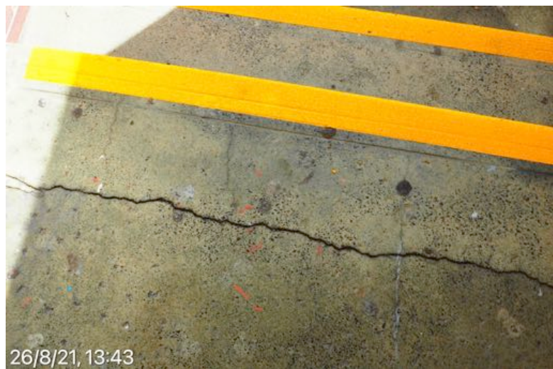
MOSMAN HIGH SCHOOL Building D North facade centre stairs to east stairs. 26 August 2021 at 13:43:06
