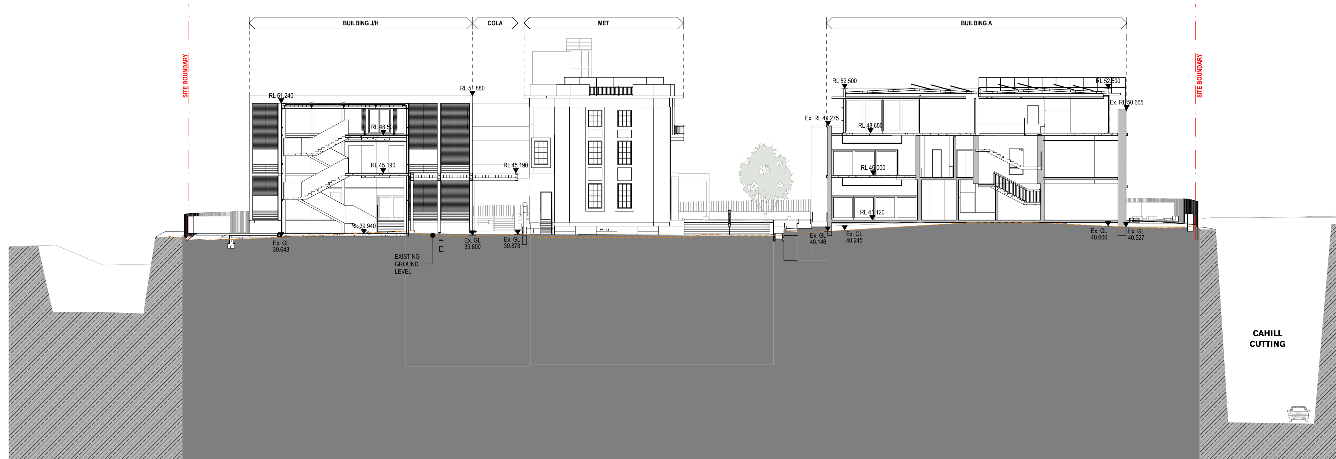
1 SECTION Section At COLA 1:200
