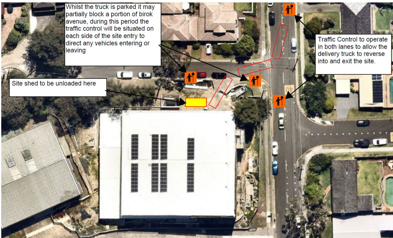
Site map showing traffic control plans
