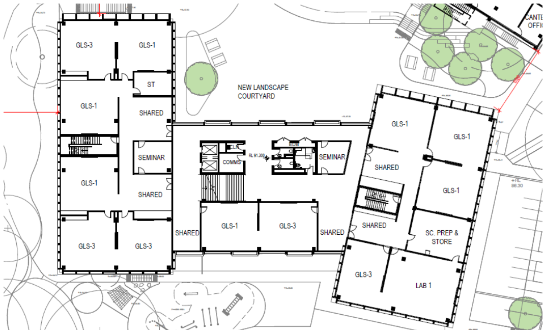
Figure 32 Building S Floorplate (at Ground Level)
