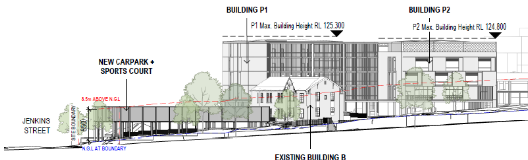
Figure 42 Southern elevation of P1 and P2 indicating 8.5 metre height limit (red line)
