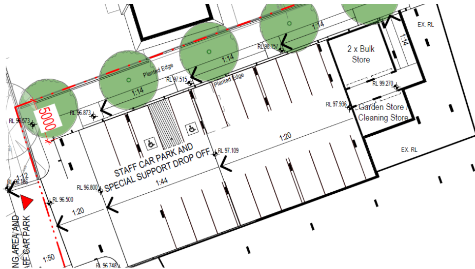
Figure 29 Car park layout (sports court above) (at Lower Ground Level)
