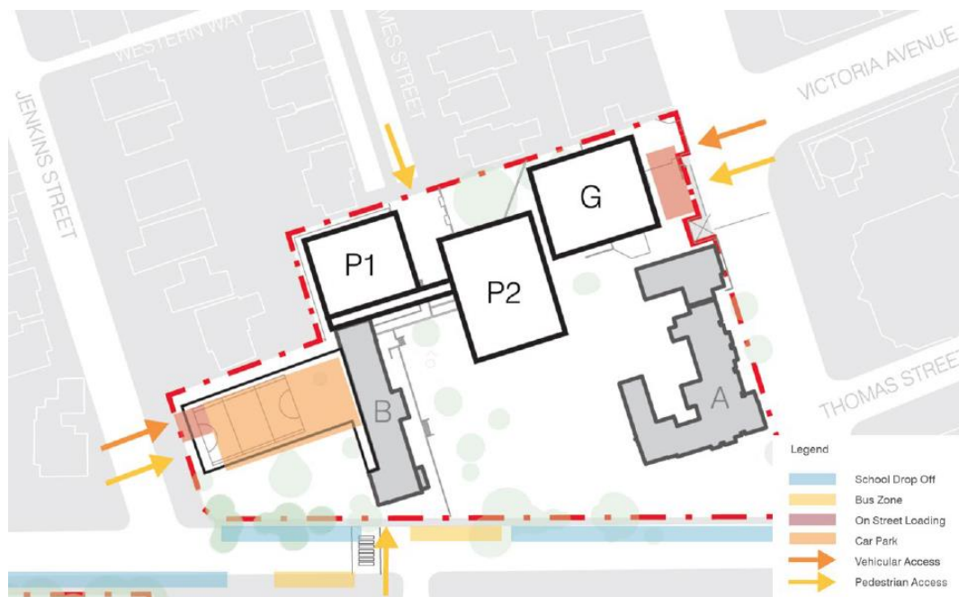
Figure 58 Proposed vehicle and pedestrian access arrangements
