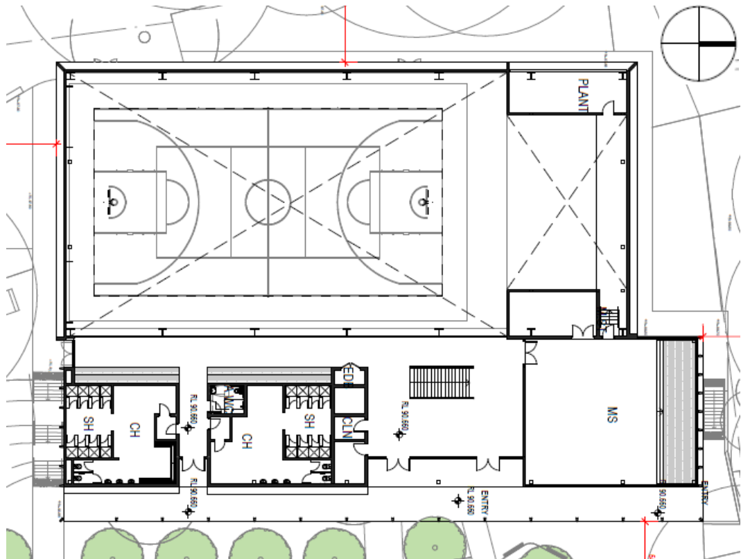
Figure 33 Building T Floorplate (at Ground Level)
