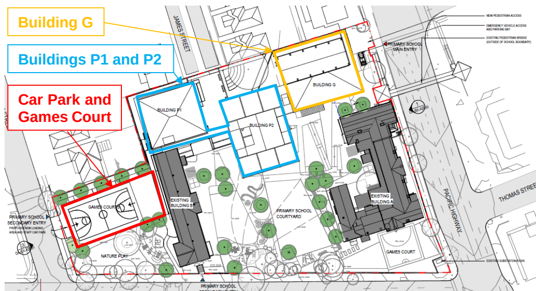
Figure 26 Proposed site plan for Chatswood Public School
