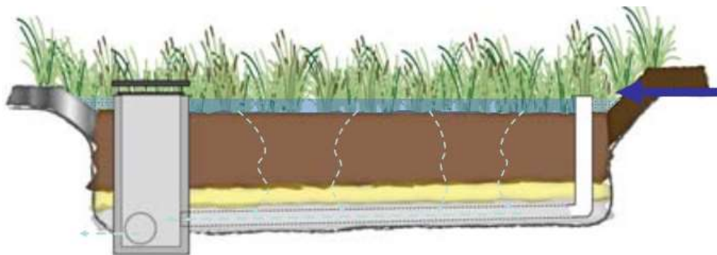
Figure 14: Typical Section of a generic Bio-Detention system (Source: Water by Design)
