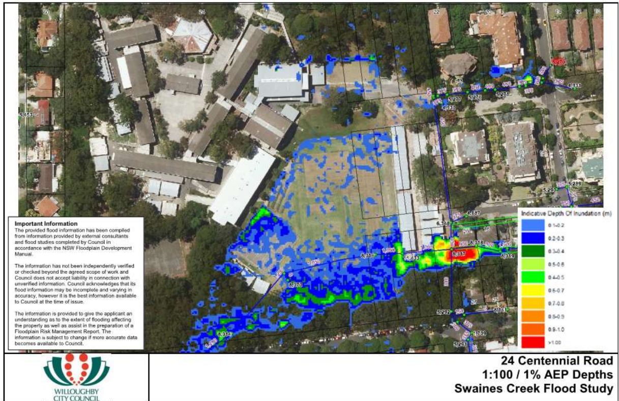
Figure 8 – TUFLOW Model Results 1% AEP (Source: Willoughby Council)
