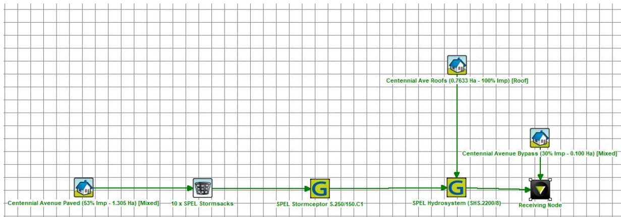
Figure 16 – MUSIC Model Centennial Avenue Site
