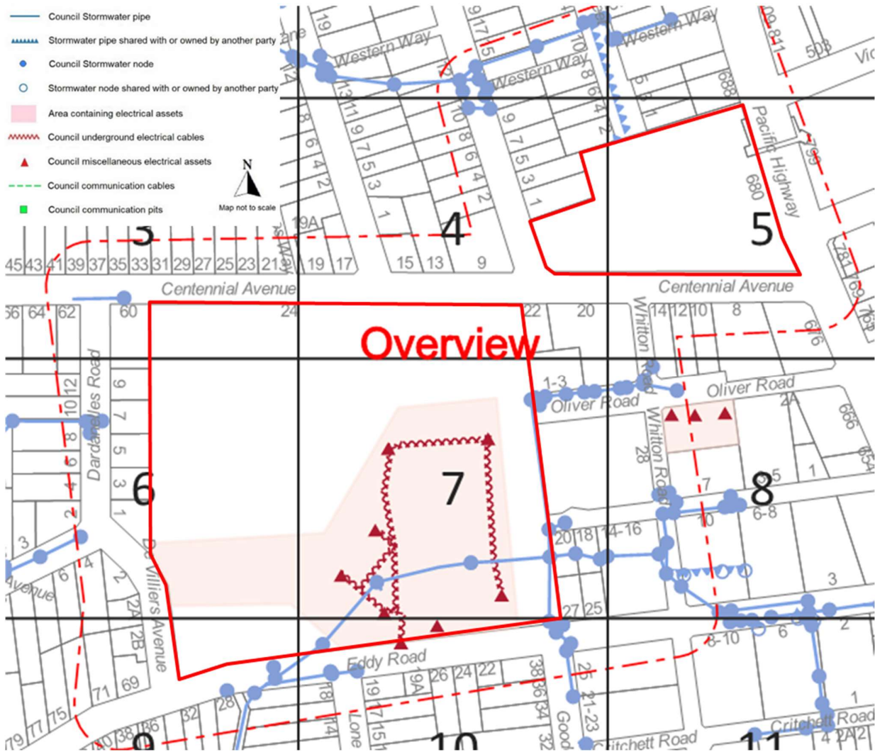
Figure 5 - Internal Site Catchment
