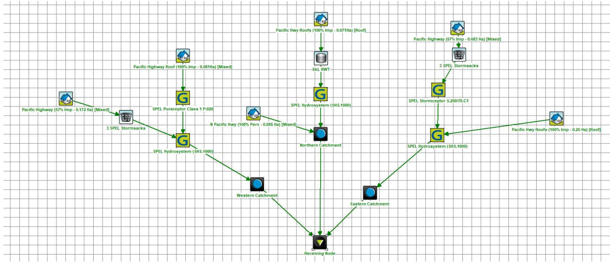
Figure 15 – MUSIC Model Pacific Highway Site
