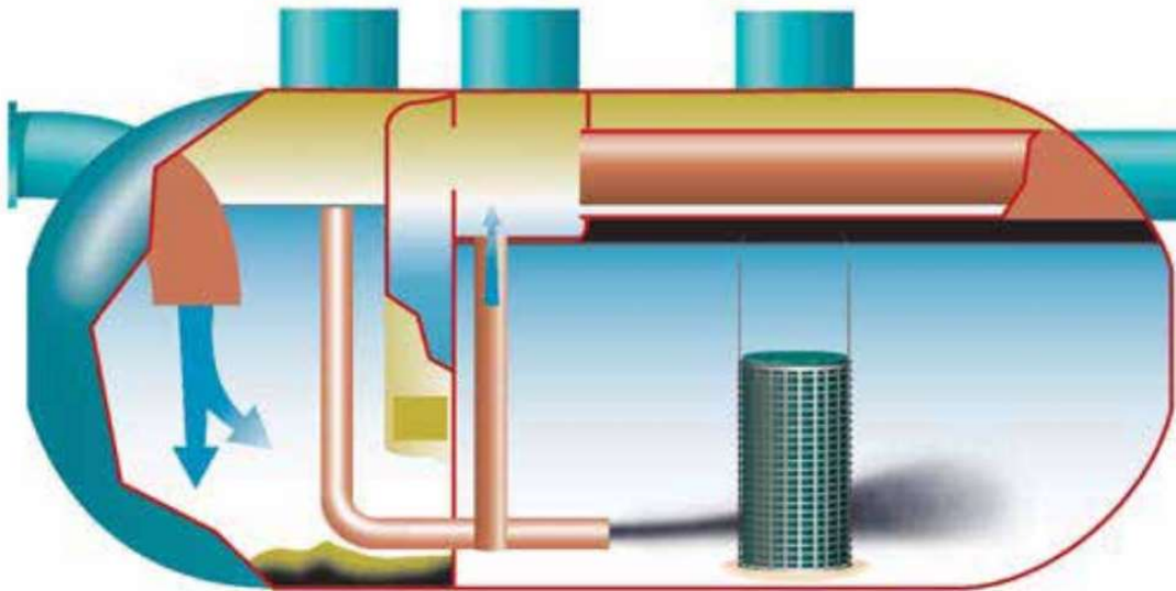
Figure 13 – Puraceptor Unit (Source: SPEL Stormwater)
