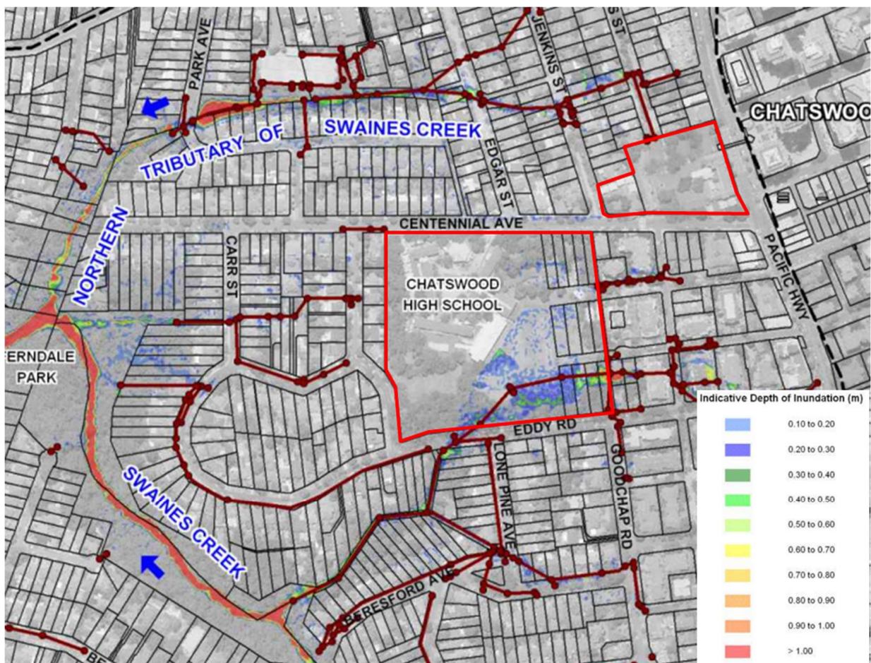
Figure 7 – TUFLOW Model Results 100YEAR ARI (Source: Swaines Creek Flood Study, March 2014)
