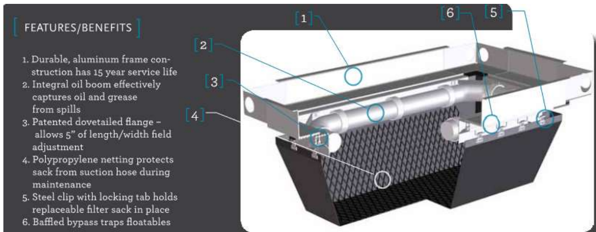
Figure 11 – Stormsack Pit Inlet Trap (Source: SPEL Stormwater)
