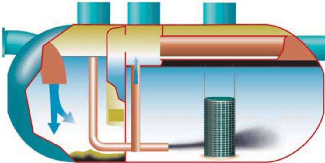
Figure 12 – Stormceptor Unit (Source: SPEL Stormwater)
