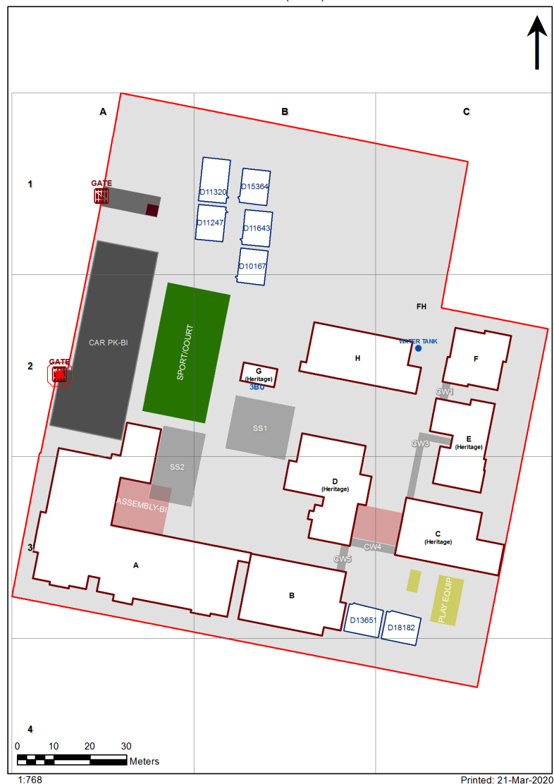
7424 - Liverpool Public School Site Plan (11543)
