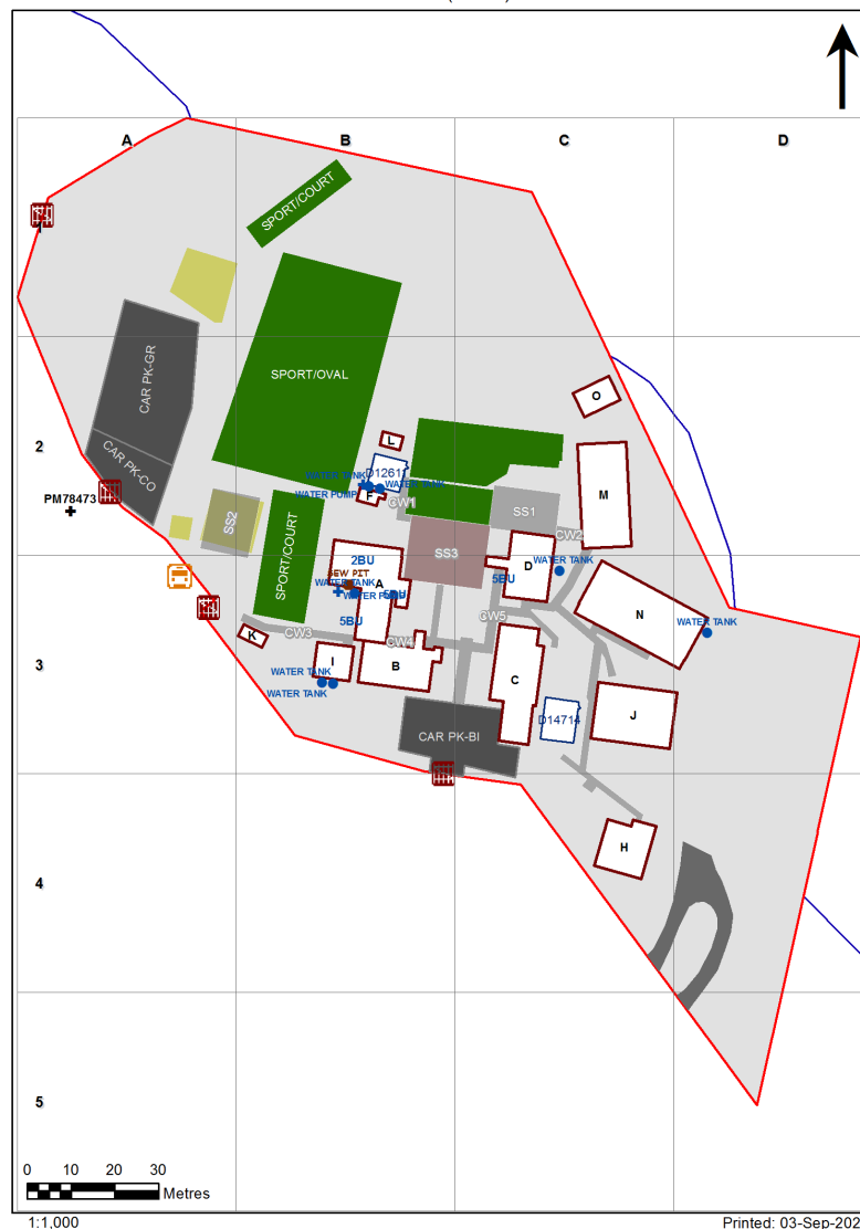
2407 - Lisarow Public School Site Plan (12769)
