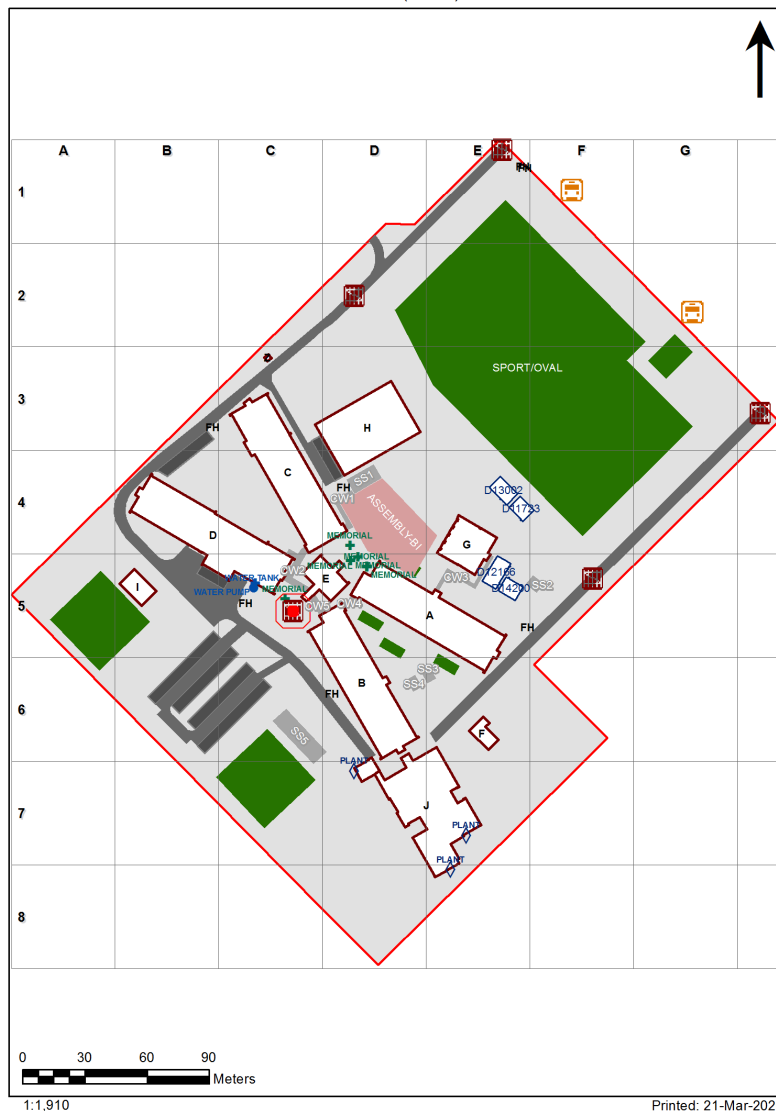
8262 - Ingleburn High School Site Plan (10758)
